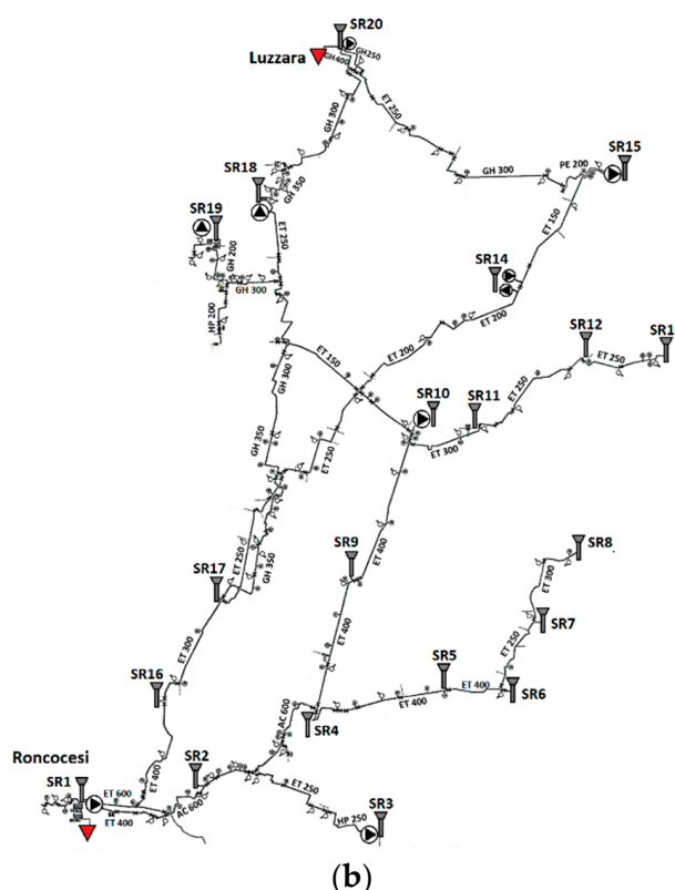
Figure 3. (a) Districts served by Roncocesi and Luzzara networks; (b) Schematization of Roncocesi and Luzzara networks, with main components.
