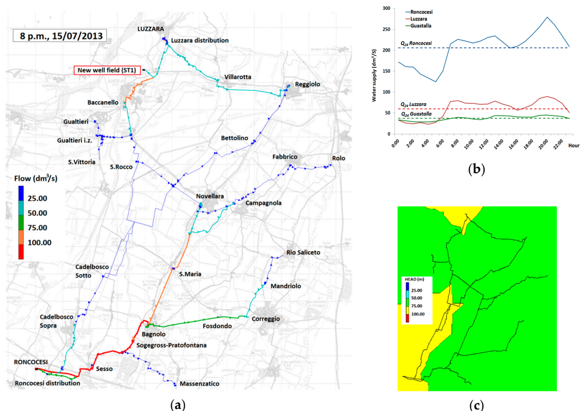
Figure 7. Hydraulic simulations of ST1 over the day of highest consumption (15 July 2013). (a) Flows derived at 8 p.m. (b) Average hourly water supply ( \text{dm}^3/\text{s} ) introduced in Roncoresi, Luzzara, and Guastalla networks by the main reservoirs; (c) Contour plot of the total head over the networks at 8 p.m.
